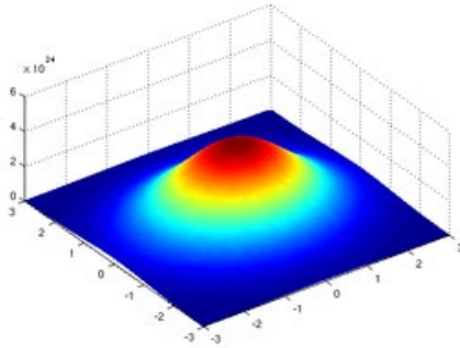
Figure 3. Two Dimensional Gaussian Distribution
