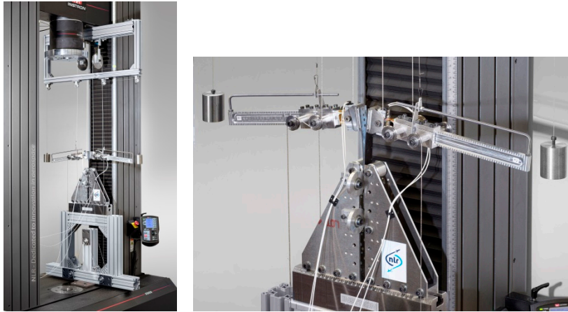
Figure 9: Moment loading cantilever beam setup. This will enable a-symmetric coupons to be testing in Mode I, Mode II and mixed modes with constant moment. The load is applied by the arms which are loaded by the steel cables
