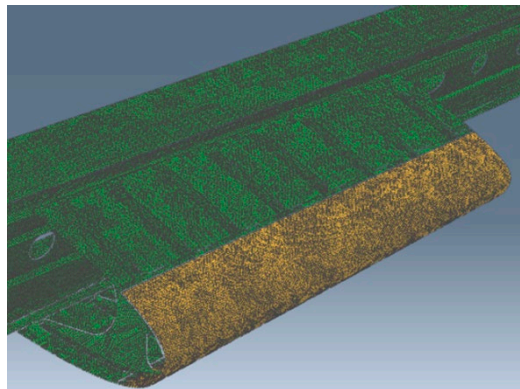
Figure 2. Model of the bonded thin titanium sheet (yellow) over the CFRP structure designed for Hybrid Laminar Flow Control (HLFC)
