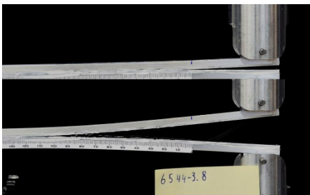
Figure 6: (left) figure of the DCB setup with TicoAjo coupon. (right) the load – displacement curve of the six DCB coupons tested. The peaks in the beginning are the settling of the test-setup joints
