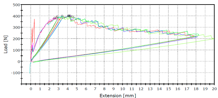
Figure 6: (left) figure of the DCB setup with TicoAjo coupon. (right) the load – displacement curve of the six DCB coupons tested. The peaks in the beginning are the settling of the test-setup joints
