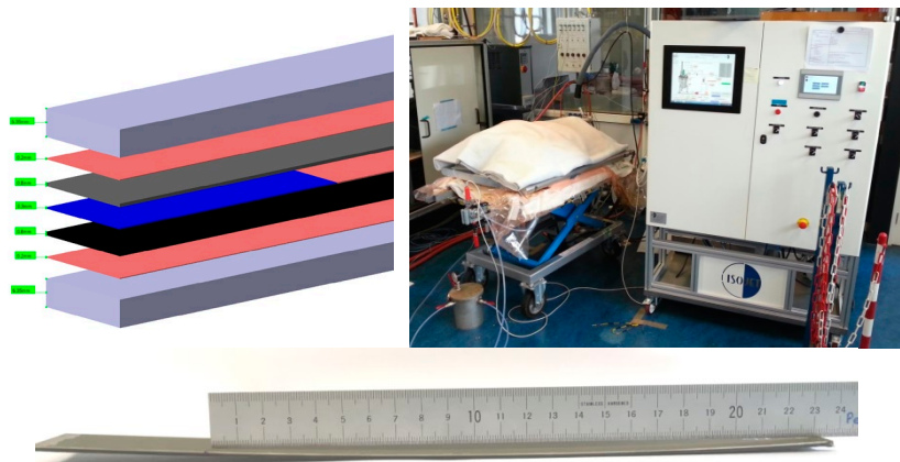
Figure 3: (left) image of the coupon composite with the backing material, adhesives, titanium and composite. The blue layer is the Upilex foil. (Right) the VARTM process. (bottom image) Finished Ti-CFRP coupon without the backing plates where the curvature is clearly visible. The titanium is on the upper side, the CFRP on the lower side. The titanium has a larger coefficient of thermal expansion and shrinks more during cooldown
