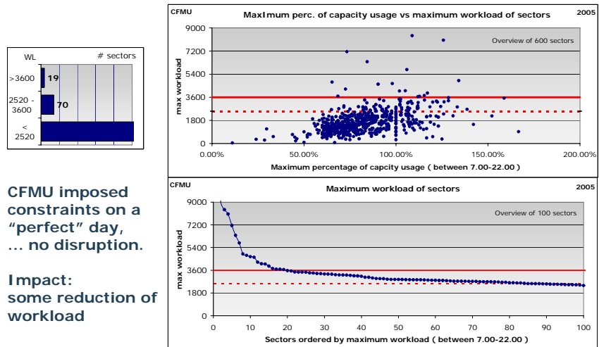
Figure 7 Reference data of maximum traffic load against workload per sector after CFMU regulations (2005)
