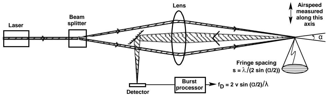
Figure 3: Dual-beam laser Doppler configuration.
