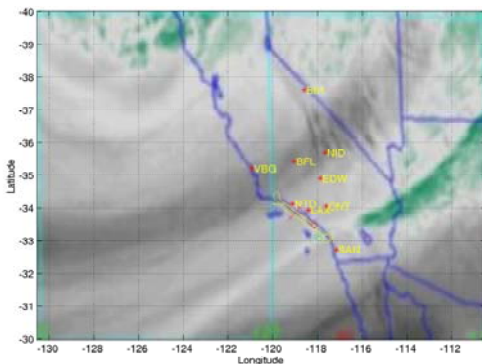
Figure 7: Weather map showing bands of moisture concentrations on the California-Nevada border indicating mountain rotor conditions [30].
