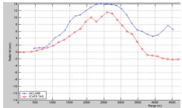
Figure 8: Chart showing lidar airspeed (blue) and conventional airspeed comparison in the mountain rotor region [30].
