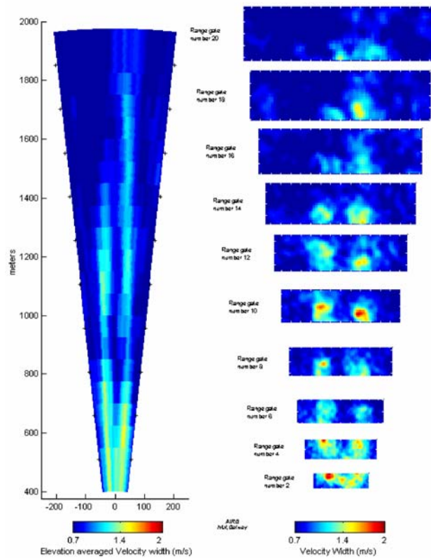
Figure 11: Wake vortices detected with I-Wake / MFLAME detection system.
