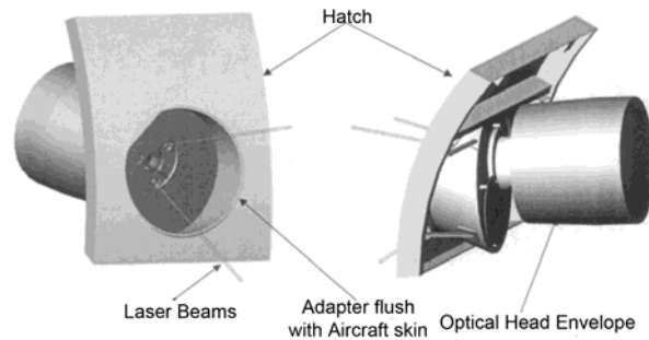
Figure 10: MOADS Optical Head showing three laser beams projected into the measurement region to the side of the aircraft [32].
