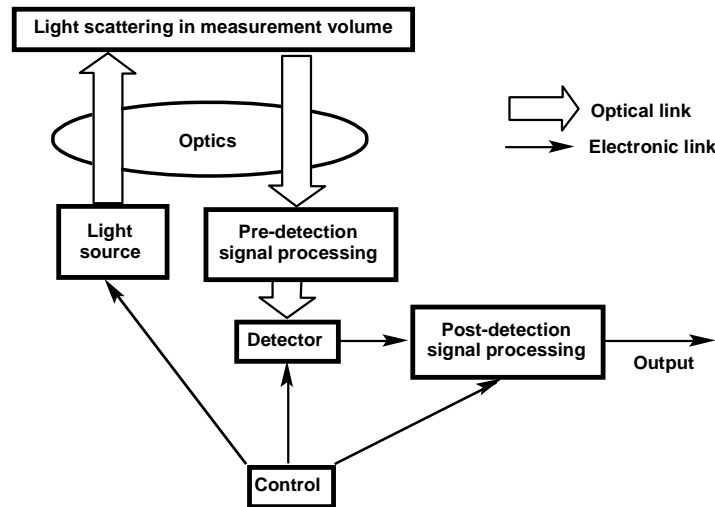
Figure 1: Generic block diagram of an in-flight flow measurement system.
