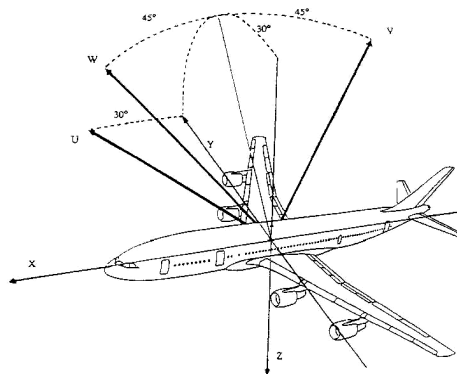
Figure 4: Line-of-sight measurement in three directions to derive true airspeed, angle of attack and angle of sideslip for calibrating the air data system.
