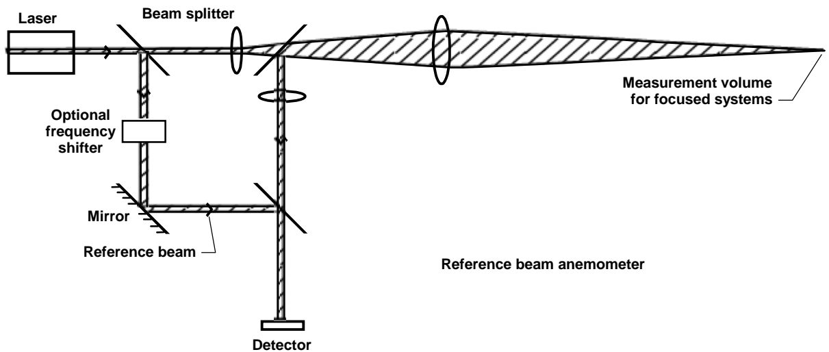
Figure 2: The reference beam in backscatter configuration.
