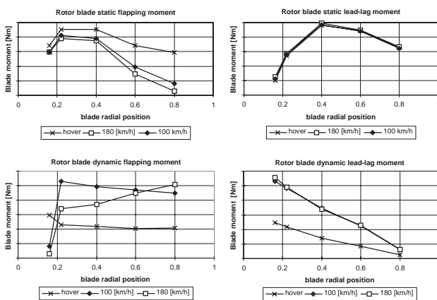
Fig. 11 - Sample rotor blade radial load distribution at C_T=0.007
