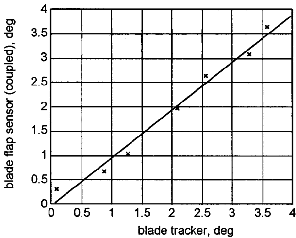
Fig. 13 - Blade coning angle measurement accuracy
