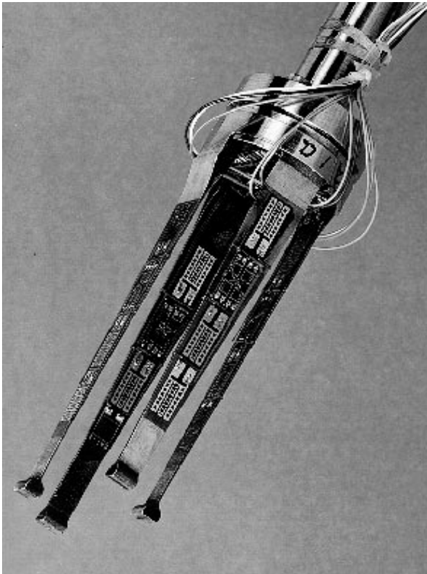
Fig. 3 - Blade angle measurement system (photo: NLR)
