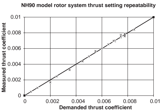
Fig. 14 - Repeatability of thrust setting
