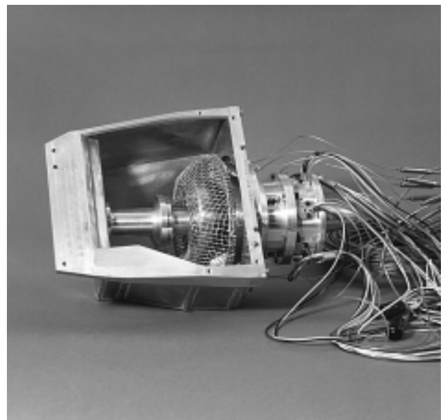
Fig. 4 - Air intake module (photo: NLR)
