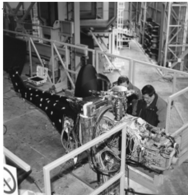
Fig. 7 - Model in DNW-LLF parking hall, fuselage skin and rotor blades removed (photo: NLR)
