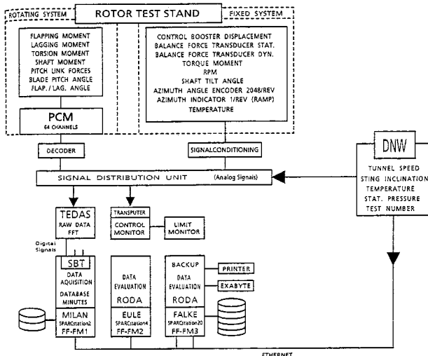
Fig. 10 - Flow diagram of DLR data acquisition and processing chain
