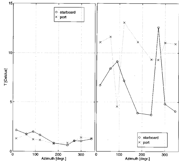
Fig. 15 - Sample air intake temperature change due to re-ingestion
