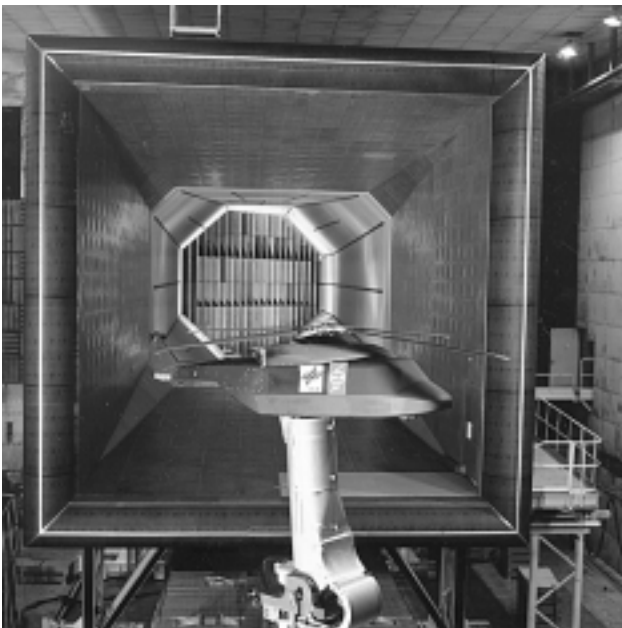
Fig. 8 - NH90 model in the open jet test section of the DNW-LLF (photo: DNW)
