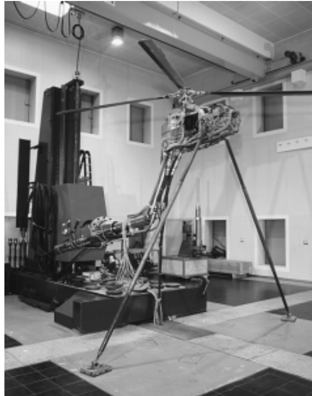
Fig. 5 - Model rotor system set up during testing at DLR Braunschweig (photo: NLR)
