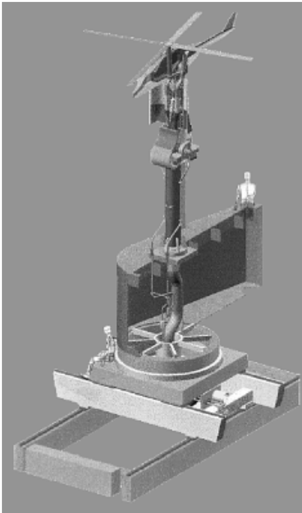
Fig. 6 - Schematic CAD/CAM model to aid assembly of the test set up
