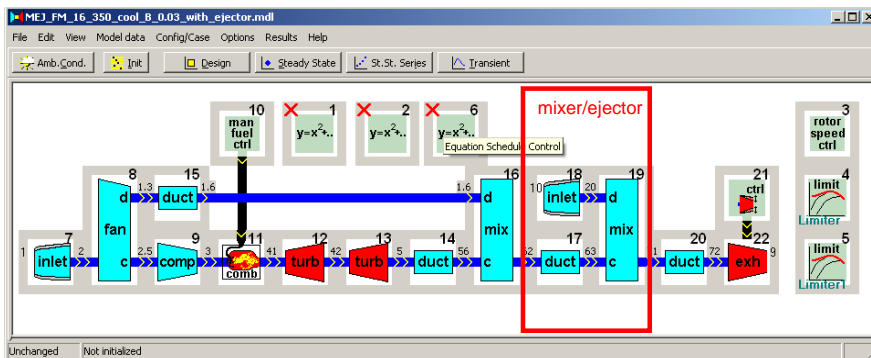
A turbofan model within the NLR Gas Turbine Simulation Program GSP with a supersonic mixer-ejector
