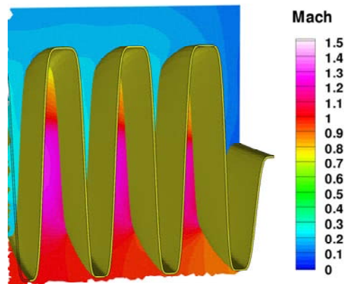
Fig.2 Mach number distribution in the forced mixer calculated with the NLR Euler code (NLR, Laban)
