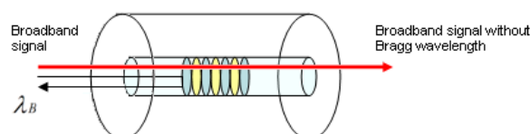
Figure 3 Fibre Bragg Grating concept
