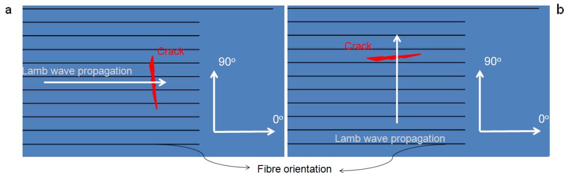
Figure 5 (a) The Lamb wave propagates parallel with the fibres in the 0° orientation with the crack at 90° to the wave propagation. (b) The Lamb wave propagates perpendicular to the fibres in the 90° orientation with the crack at 0° to the wave propagation
