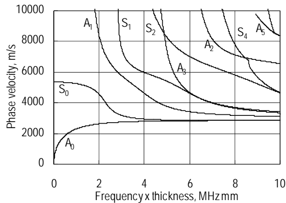
Figure 2 The dispersion curve of an 1mm thick aluminium plate. The antisymmetric (A) and the symmetric (S) waves are plotted, including the higher modes ENREF 4 .
