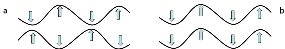
Figure 1 Configuration a represents the zero-mode symmetrical wave ( S_0 ). In configuration b the antisymmetrical wave ( A_0 ) is shown.
