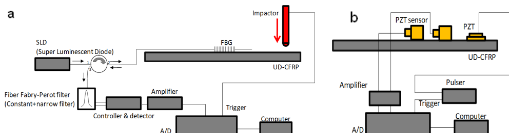
Figure 4 Schematic over view of the experimental setups. (a) shows the FBG setup and (b) the setup for the verification measurements with PZT sensors
