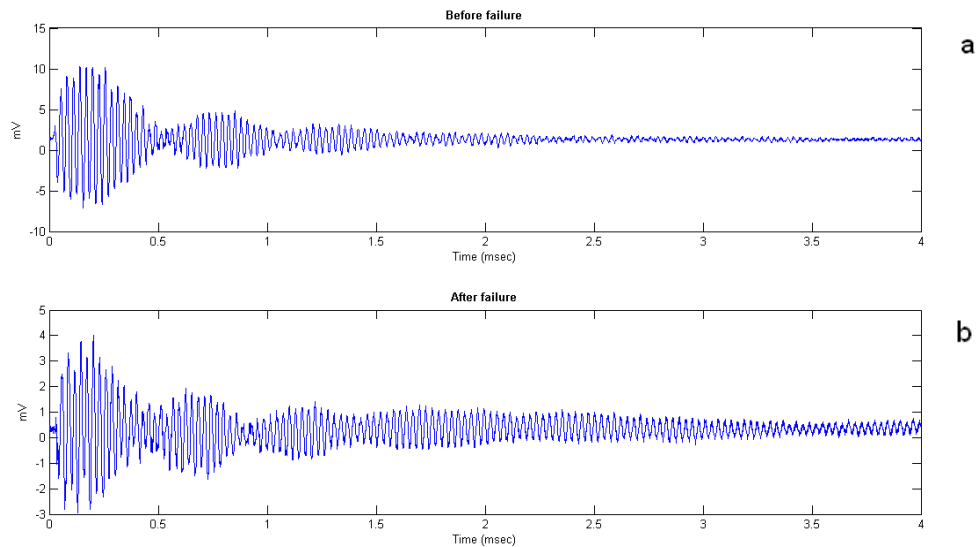
Figure 8 Wave measurements before (a) and after (b) flaw situation in a single prepreg UD-CFRP sheet are shown for the 0^\circ configuration. The crack produces a reflection of the source signal, which is shown in the bottom graph.
